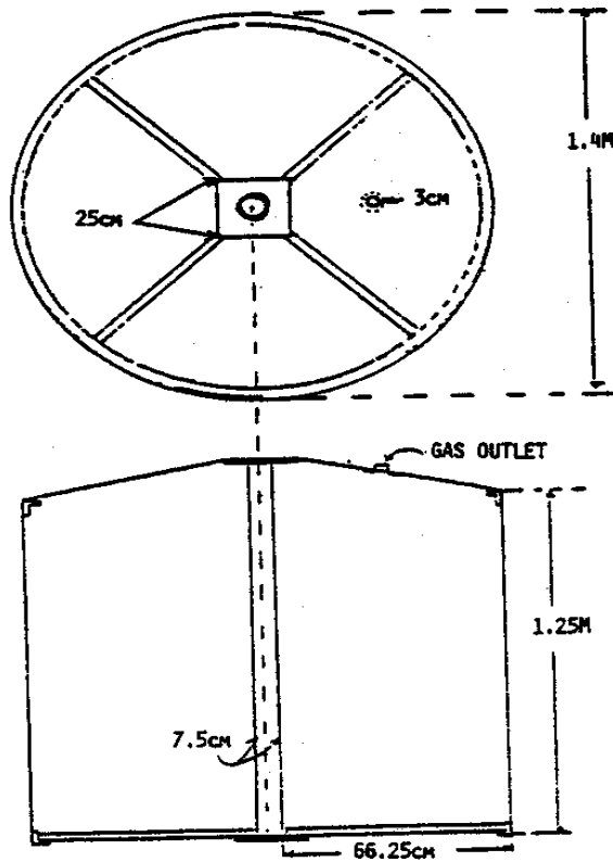
Figure 4. Biogas Plant Gas Cap
