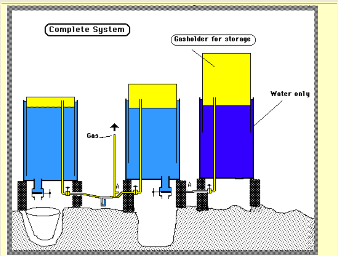
Oil Drum Biogas Digester with optional gas storage (Courtesy of E.G. Matthews)
