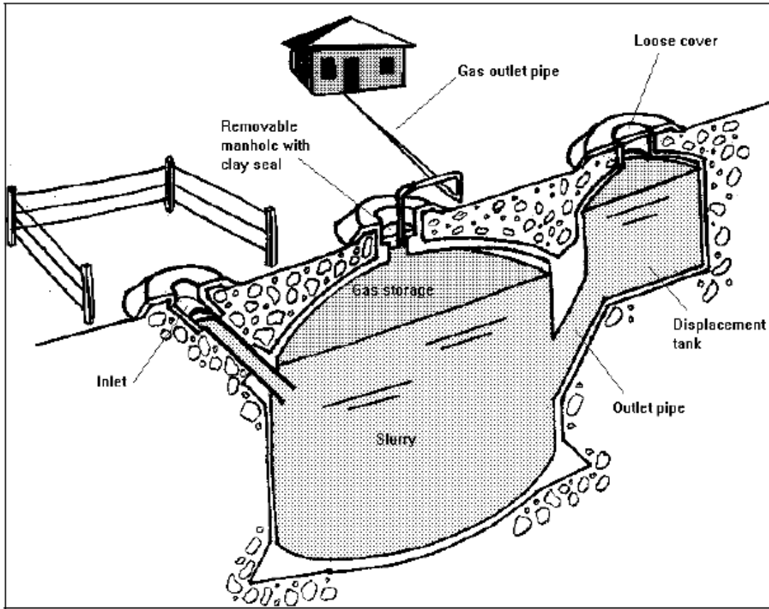
Figure 1: Fixed dome digester
